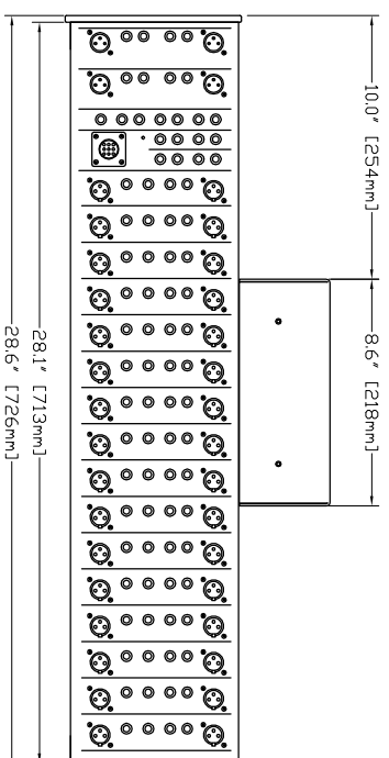
L10 Mixer 16 Channel Rear View
