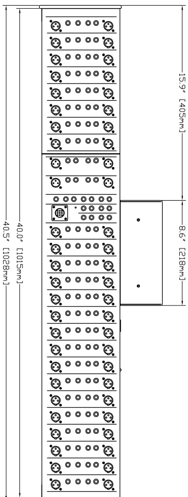
L10 Mixer 24 Channel Rear View
